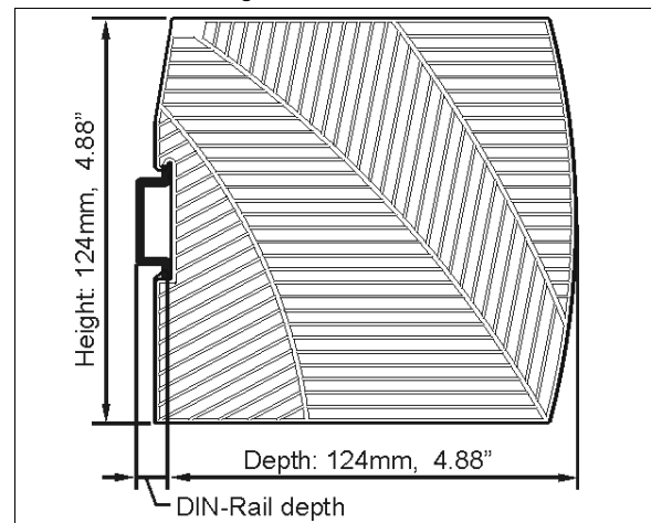
Fig. 21-2 Side view
