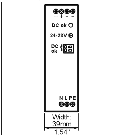
Fig. 21-1 Front view
