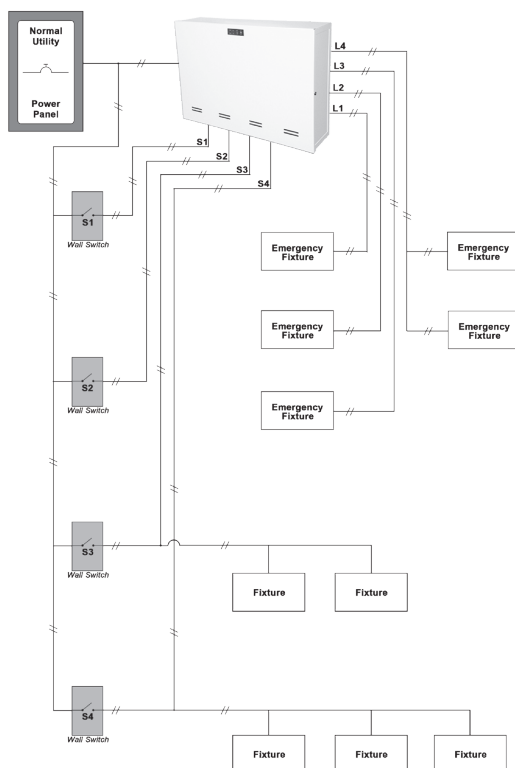
APPLICATION DIAGRAM USING 4C OPTION
